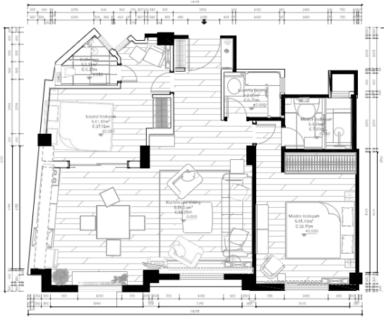
Layout Plan Drawing 1:50
