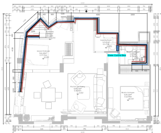
Water Supply Layout Drawing
